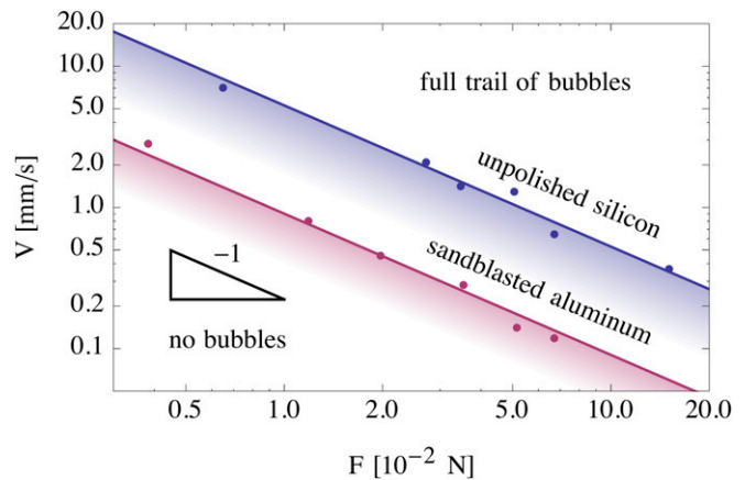
Fig. 4. Comparison between the force–velocity thresholds for unpolished silicon and sandblasted aluminum submerged in ethanol at 70 °C and having similar roughness R_a \sim 0.5 \mu\text{m} . The solid lines correspond to FV = \text{const} . In the shaded area, we still observe a partial bubble trail (Fig. 3).
