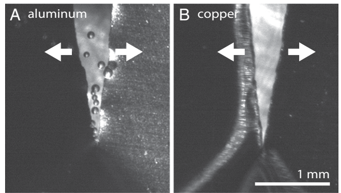
Fig. 9. Snapshots of the tearing of thin foils of (A) aluminum and (B) copper submerged in ethanol at around 78^\circ\text{C} . The foils are 12.0 and 12.5\ \mu\text{m} thick, respectively, and the two sides of the foil are torn apart with a velocity of about 9\text{ mm}\cdot\text{s}^{-1} . For aluminum, bubbles form at the tip of the tear, whereas for copper no bubbles form.
