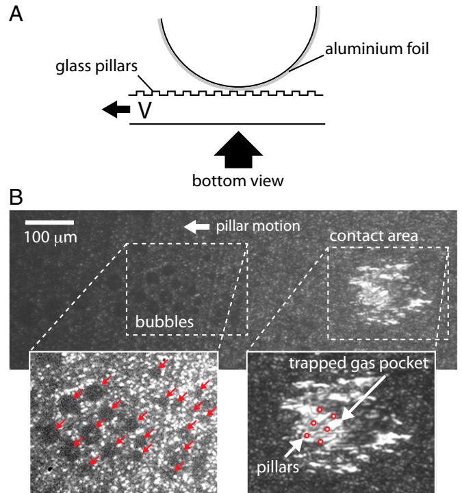
Fig. 6. (A) Schematic of the setup: a transparent glass surface covered with micropillars is rubbed against a bead covered with aluminum foil ( F = 7 \times 10^{-2} \text{ N} , V = 4.7 \text{ mm}\cdot\text{s}^{-1} ). (B) Bottom view of the experiment through a microscope. Gas pockets are trapped between the two solids in the contact area, and microscopic gas bubbles (red arrows) are observed downstream. The spacing between the pillars, their diameter, and their height are 10 , 9 , and 0.3 \mu\text{m} , respectively.
